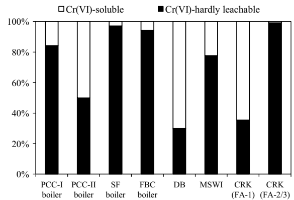
Fig. 4. Chromium(VI) speciation in fly ashes generated in the real solid fuel furnaces.
