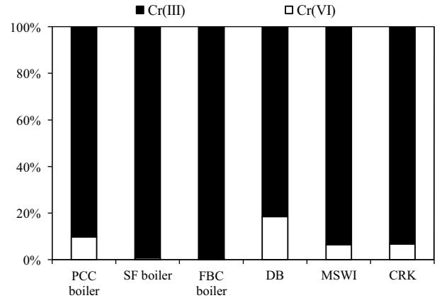
Fig. 3. Chromium valence speciation in fly ashes generated in real solid fuel furnaces based on various combustion technologies.
